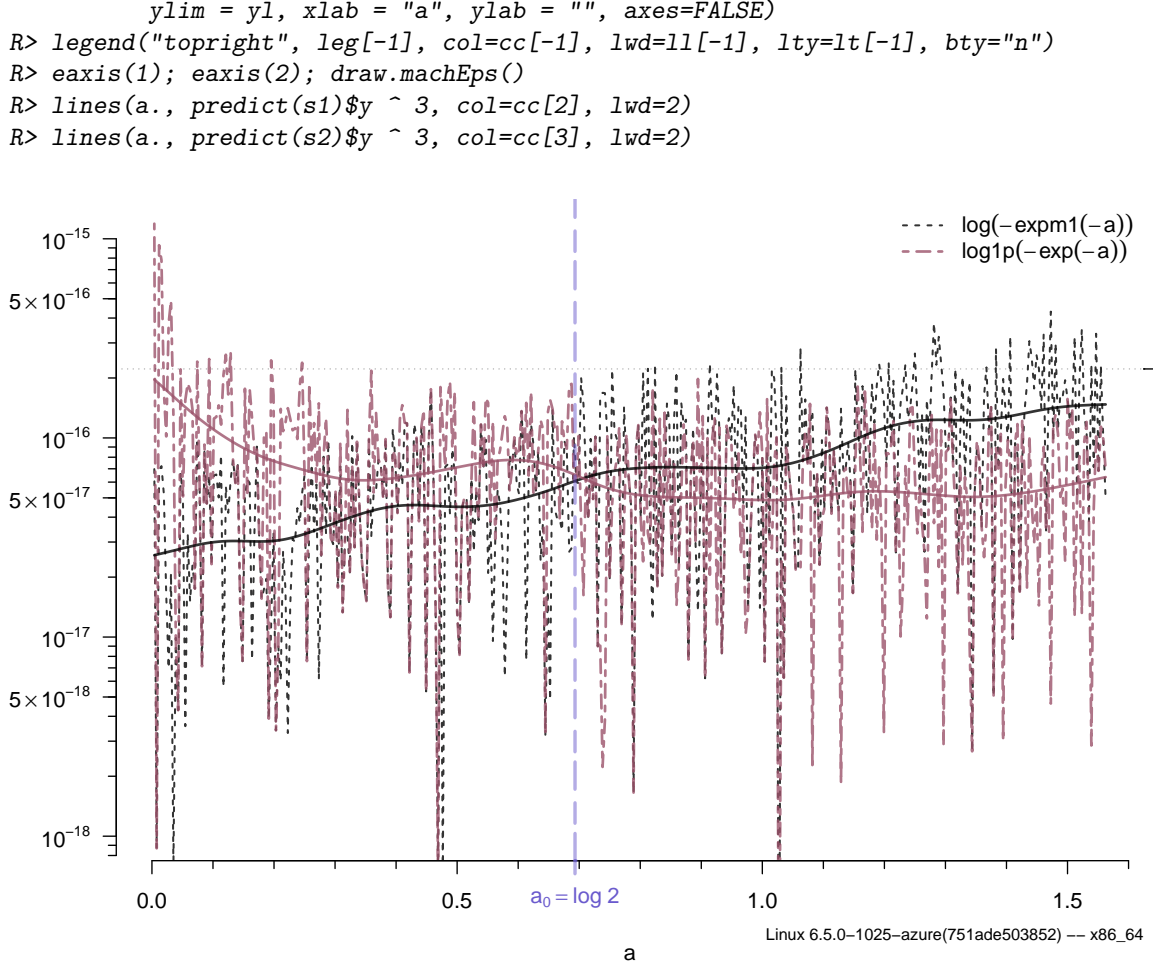
Figure 2: A “zoom in” of Figure 1 showing the region where the two basic methods, “ expm1 ” and “ log1p ” switch their optimality with respect to their relative errors. Both have small relative errors in this region, typically below \varepsilon_c := \text{Machine}\$double.eps = 2^{-52} \approx 2.22 \cdot 10^{-16} . The smoothed curves indicate crossover close to a = a_0 := \log 2 .
