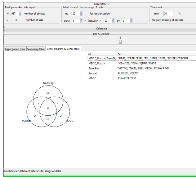
Figure 16: Venn-diagram and Venn-table results of the TopKListsGUI
