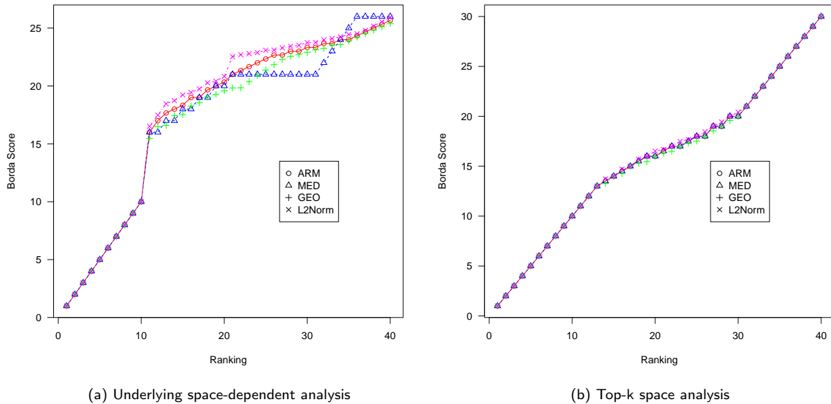
Figure 4: Plotting Borda's scores
