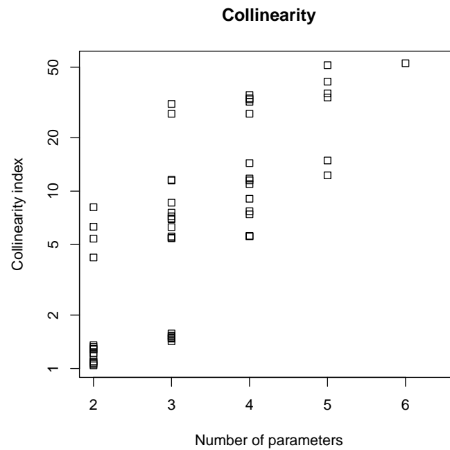
Figure 7: Collinearity plot.
