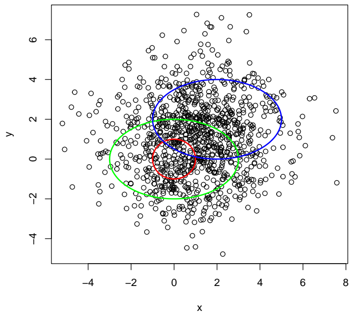
Figure 1: Independent normal noise with overlaid ellipses.
