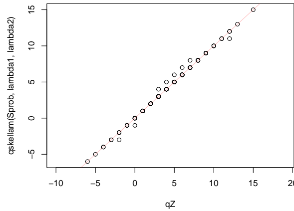
(b) quantiles
