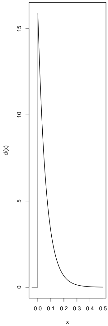
Density of AbscontDistribution
