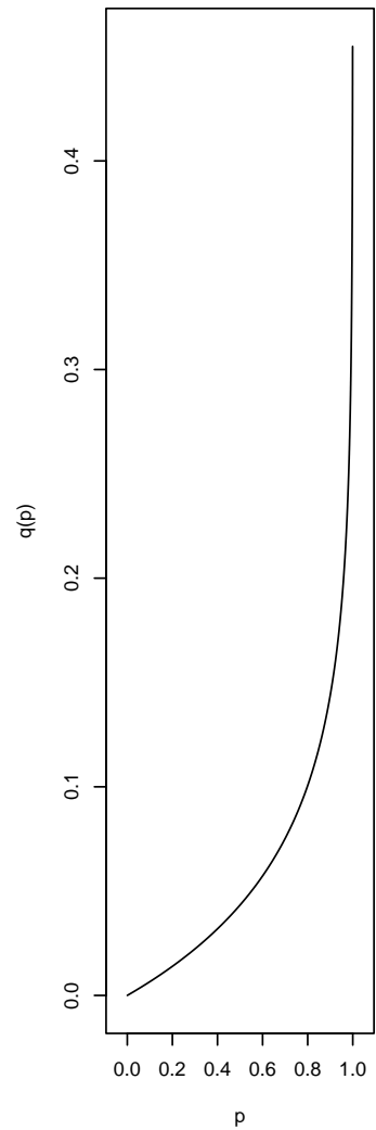
Quantile function of AbscontDistribut
