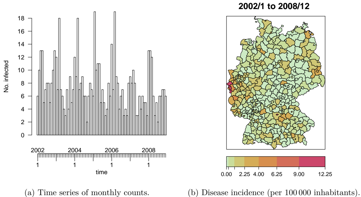
Figure 3: IMD cases (joint types) aggregated as an sts object by month and district.
